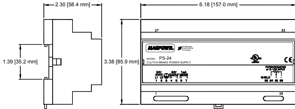
Figure 1 Enclosure Dimensions
