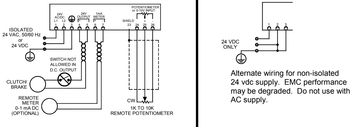
Figure 4 Electrical Connections for PS-24
