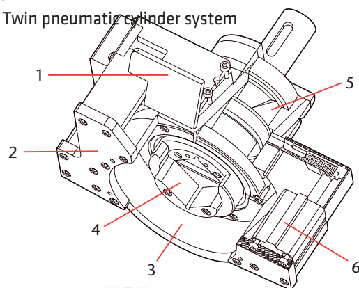
P40 Automatic Chuck
