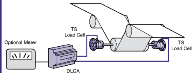
TENSION READOUT – WIDE WEB
