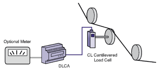
TENSION READOUT – SINGLE STRAND
