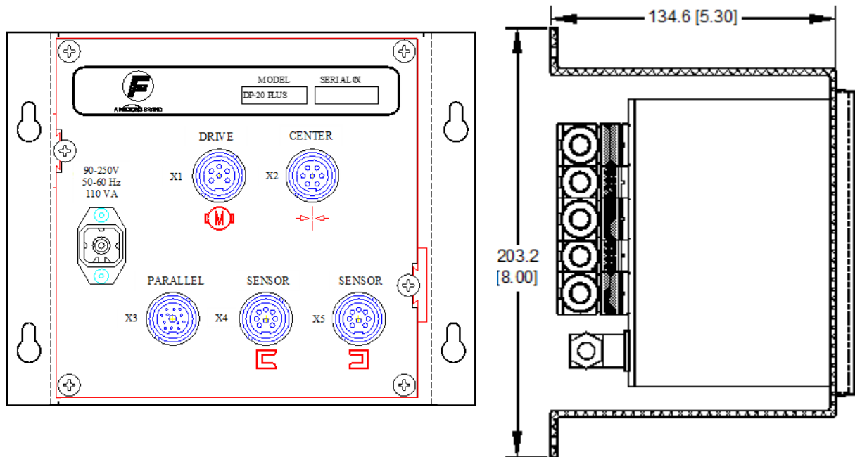
Figure 4 – Wall Mount Bracket (Rear and Bottom Views)
