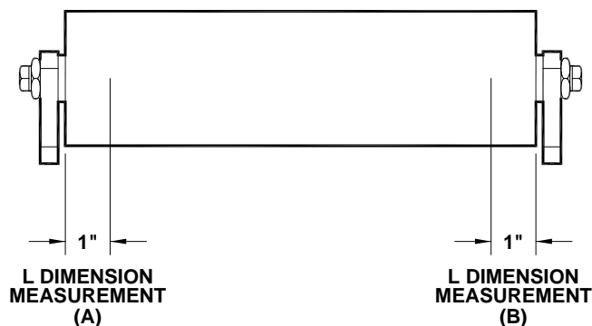
Figure 1. PIVOT CARRIER
